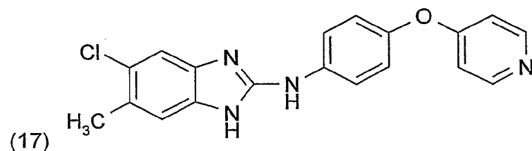
(5-Chloro-6-methyl-1H-benzimidazol-2-yl)-[4-(pyridin-4-yloxy)-phenyl]-amin
